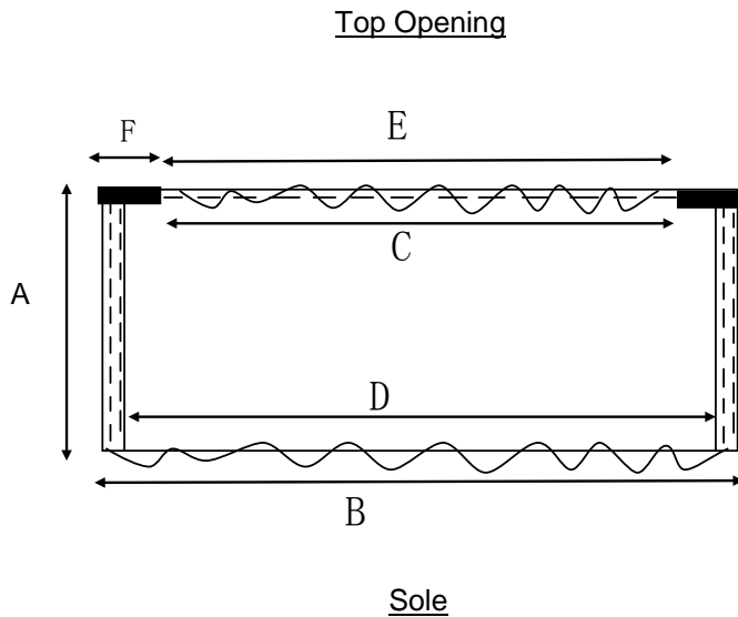
Figure 1 – Schematic representation of cover shoe measurement
